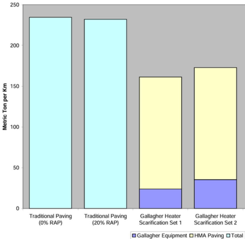
Figure 1: Comparison of Global Warming Potentials
